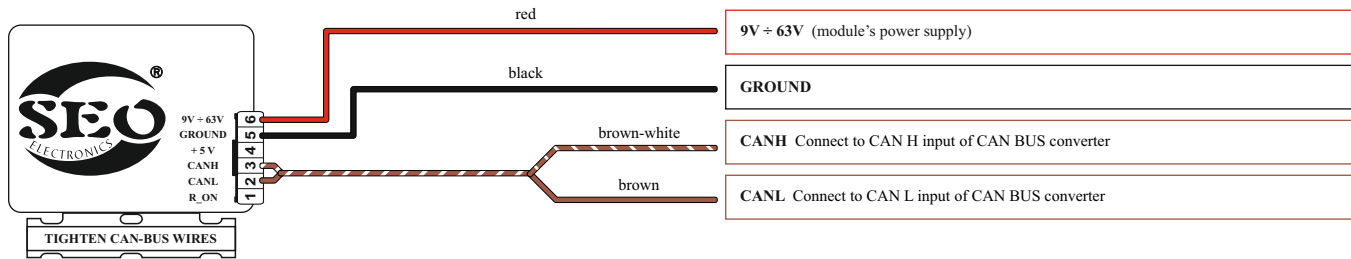
SEO CANtouch READER P400_60V
